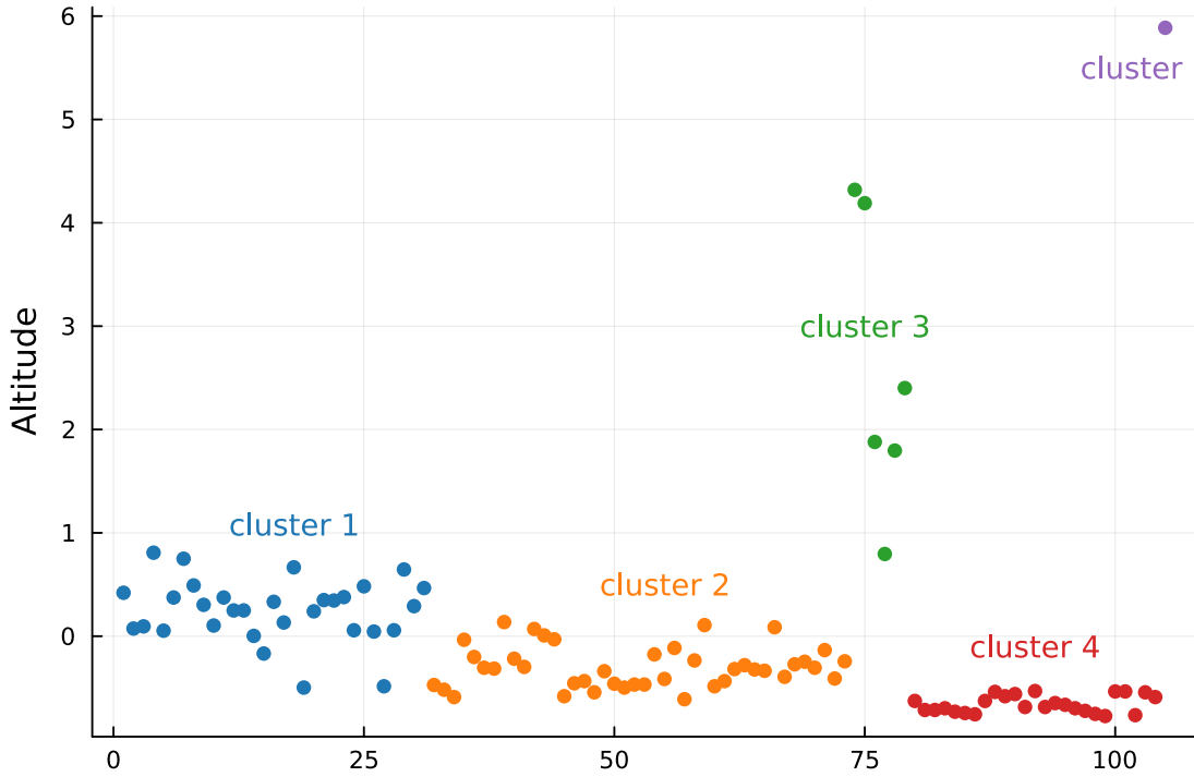
Figure 1.9: Partition considered for the covariates similarity analysis.
