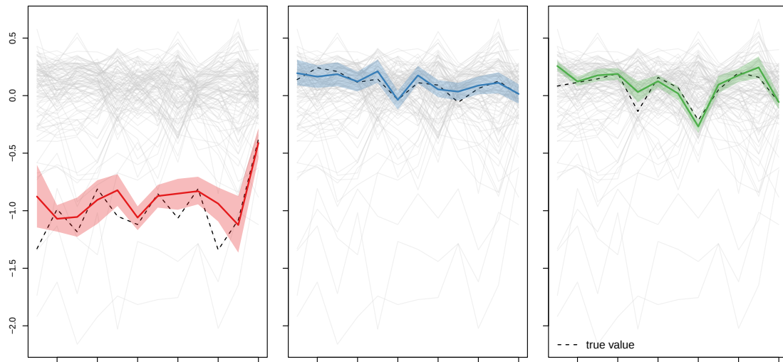
Figure 3.29: Inference analysis of JDRPM on new locations, in the spatially-informed fit with covariates in the likelihood.
