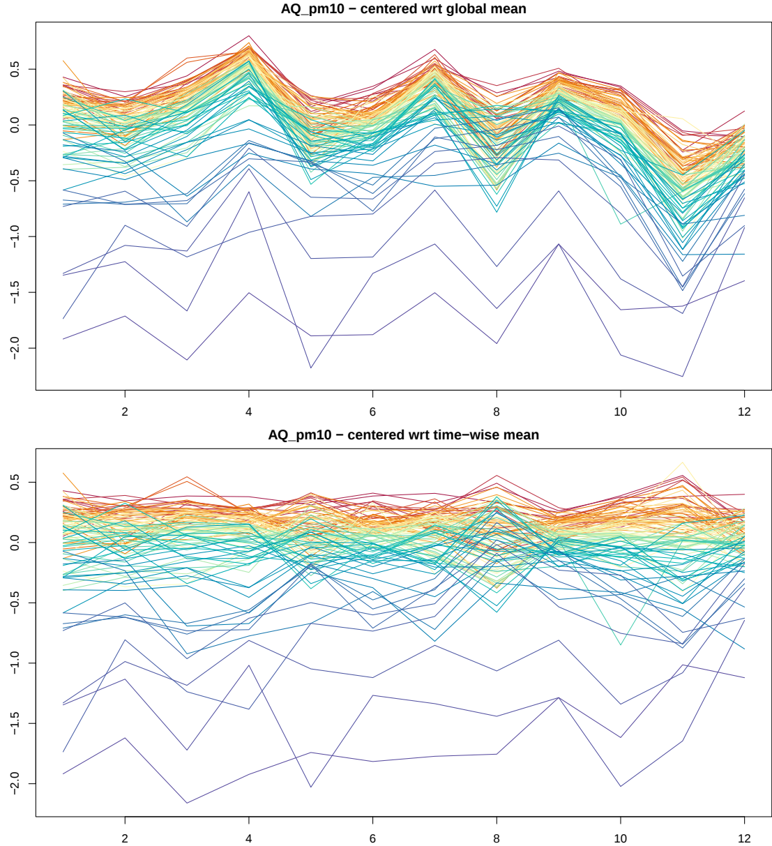
Figure 3.5: Values of the target variable AQ_pm10 adjusted using the global mean (top) and the time-wise mean (bottom). Coloring is based on the ranking of PM 10 values of the units according to their median, from highest (red) to lowest (blue).
