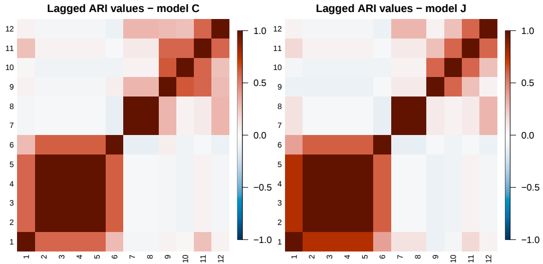
Figure 3.1: Lagged ARI values of CDRPM and JDRPM fits, in the simulated data scenario.
