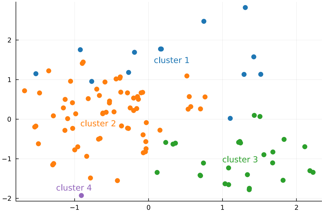
Figure 1.2: Partition considered for the spatial cohesion analysis.
